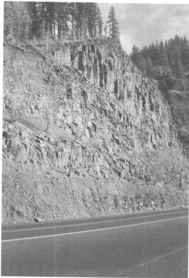
Figure 10.6 Overview of site 3. Slope height?
