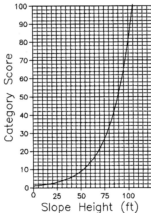
Figure 4.1 Slope height scoring graph.
