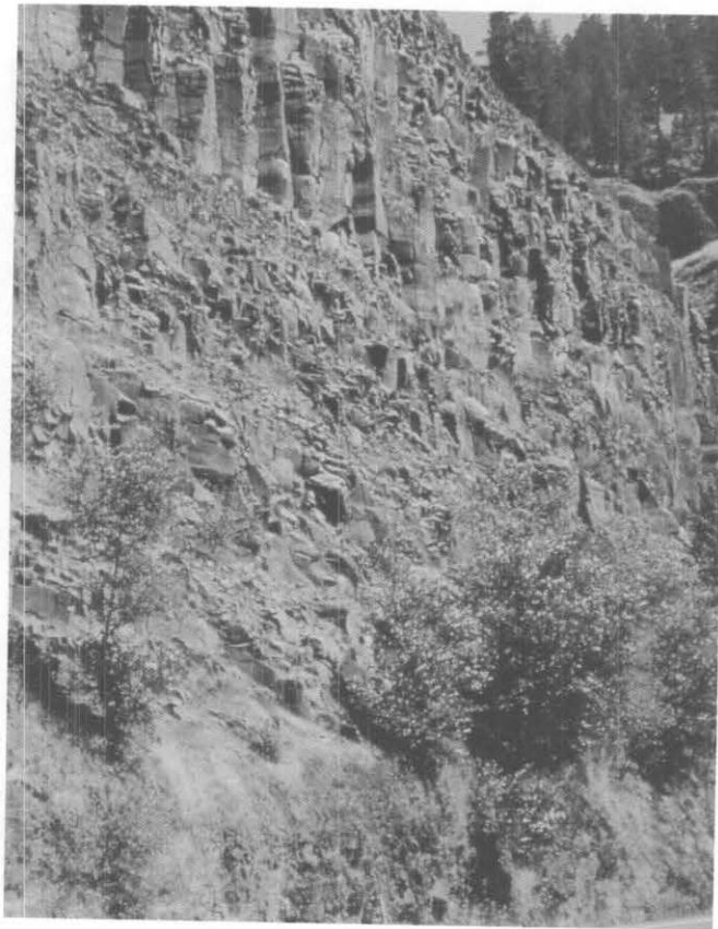
Figure 10.9 Geologic character?
