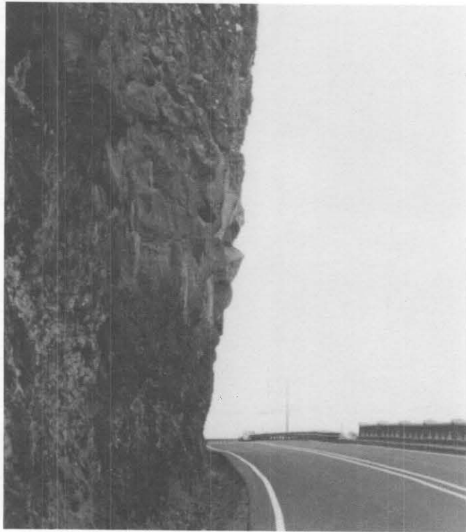
Figure 5.6 Rockfall from this slope will land on the roadway. No catchment is provided by the ditch.
