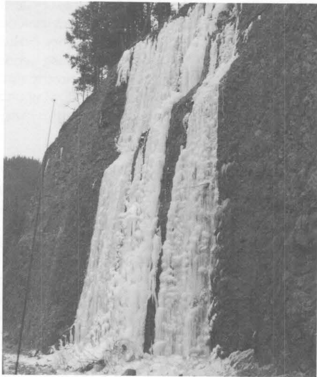
Figure 5.30 Both climate and excess water on the slope will eventually cause problems at this newly constructed site.
