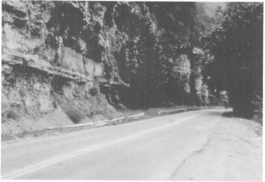
Figure 5.12 Only the width of the paved surface is rated. Note the loss of the unpaved shoulder in the distance.
