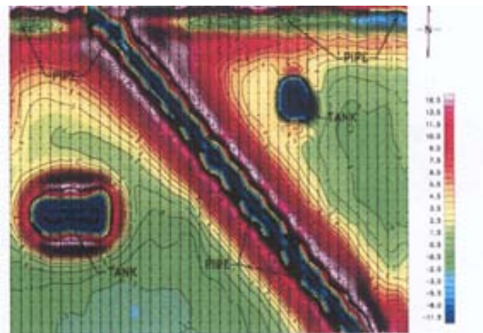
Figure 5-31. EM Survey to Detect Underground Storage Tanks (Geonics EM-31 Survey by GeoVision).
