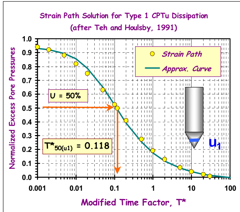
Figure 9-40a. Modified Time Factors for u_1 Monotonic Porewater Dissipations
