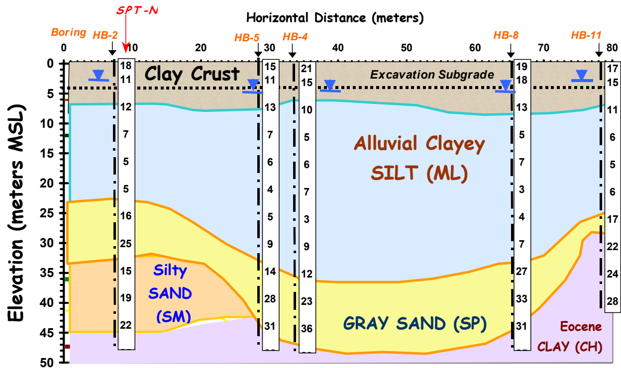
Figure 11-5. Subsurface Profile Based on Boring Data Showing Cross-Sectional View.
