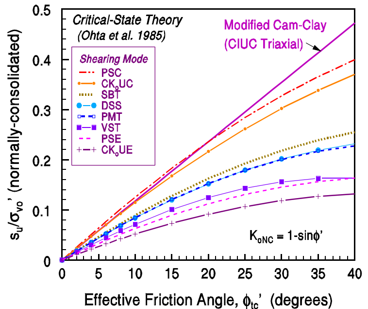
Figure 9-27. Normalized Undrained Strengths for NC Clay Under Different Loading Modes by Constitutive Model (Ohta, et al., 1985).
