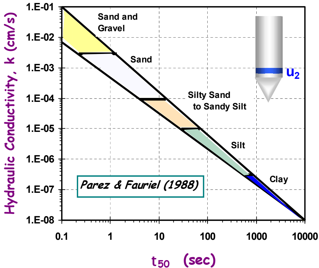
Figure 6-9: Coefficient of Permeability ( k = Hydraulic Conductivity) from Measured Time to 50% Consolidation ( t_{50} ) for Monotonic Type 2 Piezocone Dissipation Tests . (from Parez & Fauriel, 1988)
