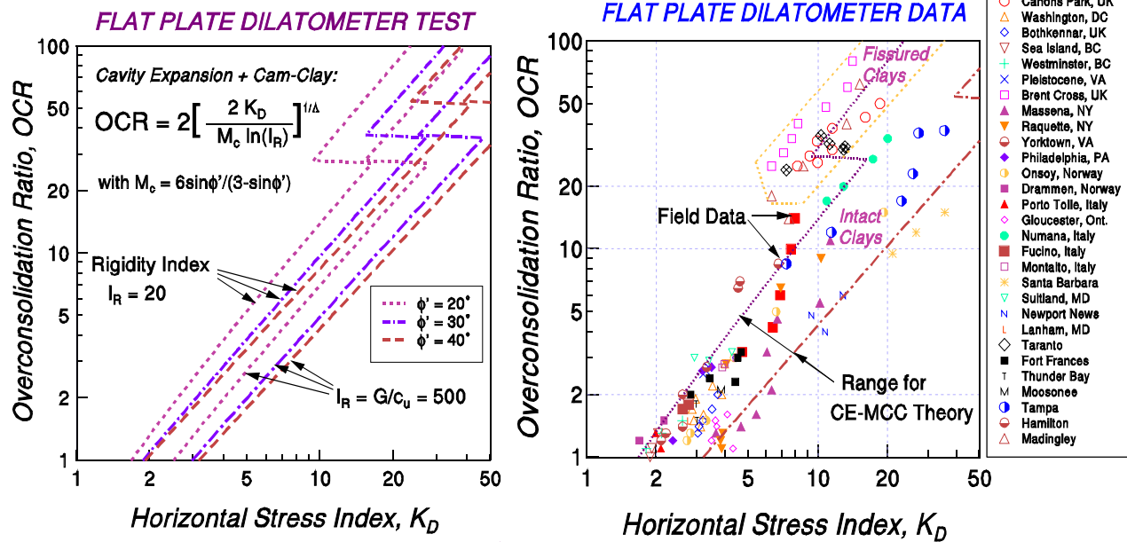
Figure 9-24. Relationships Between Overconsolidation Ratio and DMT Horizontal Stress Index, K_D from (a) Cavity Expansion-Critical State Theory, and (b) Worldwide Database from Clays
