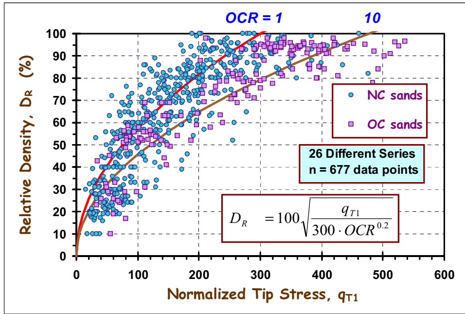
Figure 9-9. Relative Density Evaluations of NC and OC Clean Quartz Sands from CPT Data.
