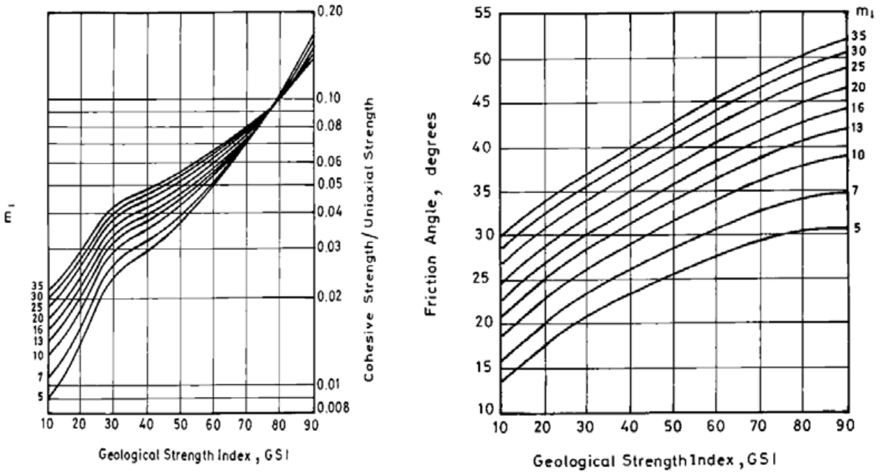
Figure 10-17. Approximate Chart Solution for Obtaining Normalized Cohesion Intercept ( c'/\sigma_u ) and Friction Angle ( \phi' ) from GSI Rating and m_i Parameter. (After Hoek & Brown, 1997).
