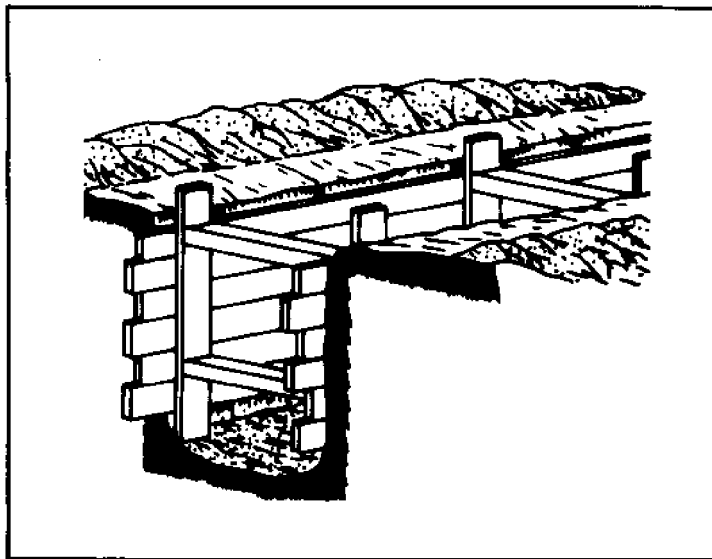
FIGURE 4 Box Shoring
